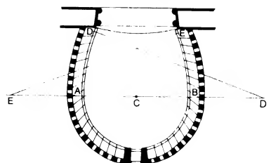
⑩ Design of the curve of the auditorium in the Teatro alla Scala in Milan
